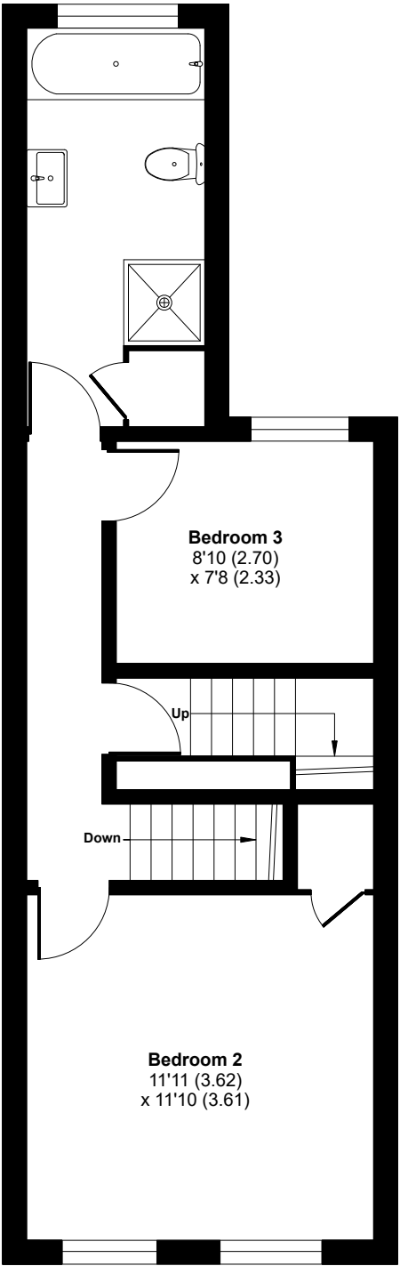
FIRST FLOOR
